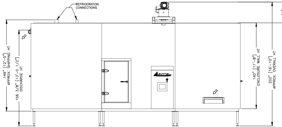
ELEVATION VIEW (CIP NOT SHOWN)
