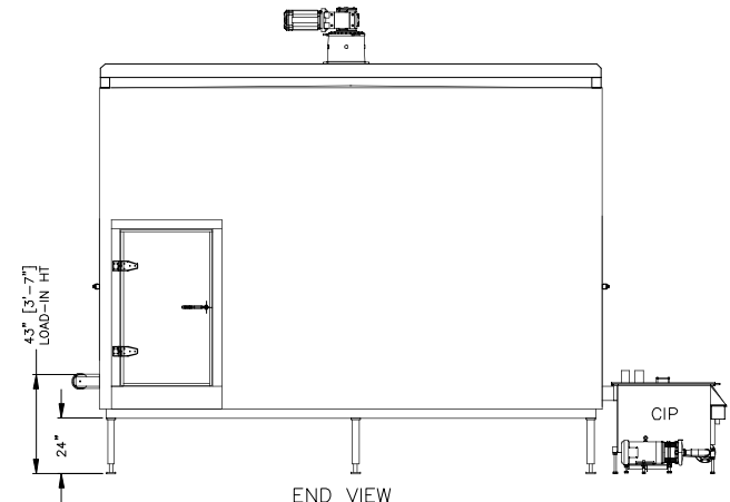
END VIEW (CONTROL PANEL NOT SHOWN)
